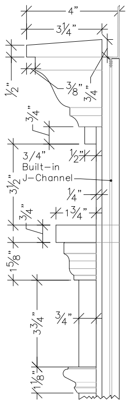
Detail #1 3"=1'-0"
