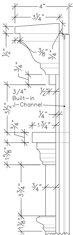
Detail #1 3"=1'-0"
