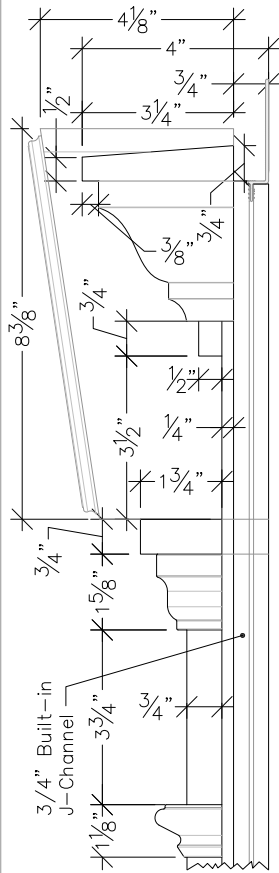
Detail #1 3"=1'-0"
