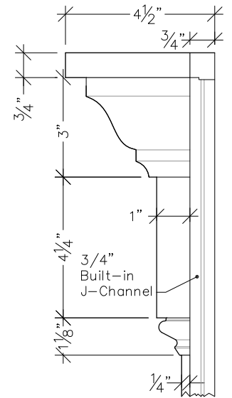
Detail #1 3"=1'-0"
