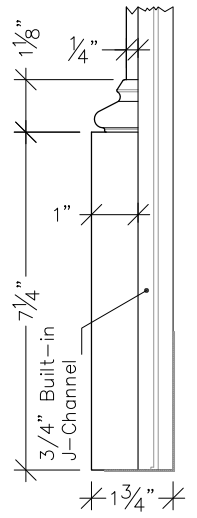
Detail #2 3"=1'-0"
