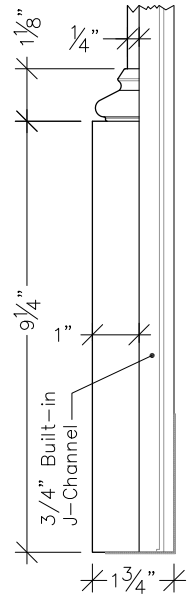
Detail #2 3"=1'-0"
