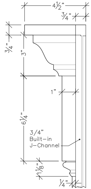
Detail #1 3"=1'-0"
