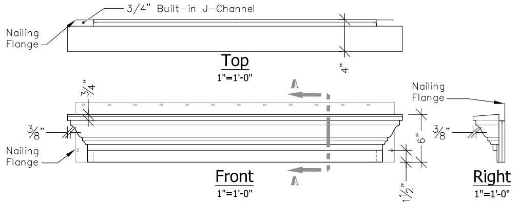
WM-1 6" Mantel
