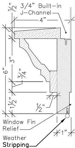
Section C-C 3"=1'-0"
