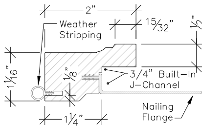
Section A-A "Brick Mould" 6"=1'-0"
