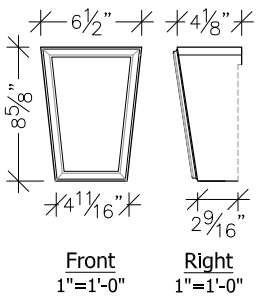
Detail #2 Keystone
