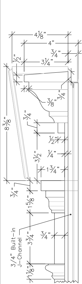
Detail #1 3"=1'-0"
