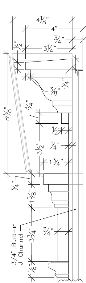
Detail #1 3"=1'-0"
