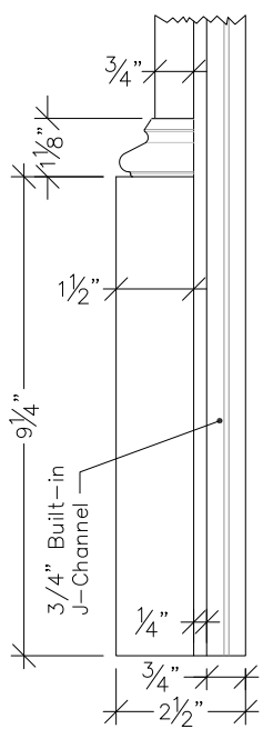
Detail #2 3"=1'-0"
