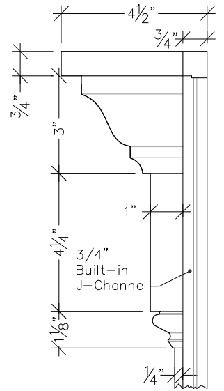
Detail #1 3"=1'-0"
