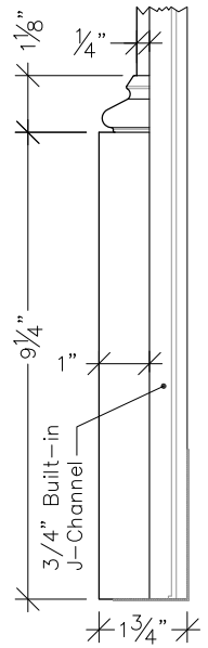
Detail #2 3"=1'-0"
