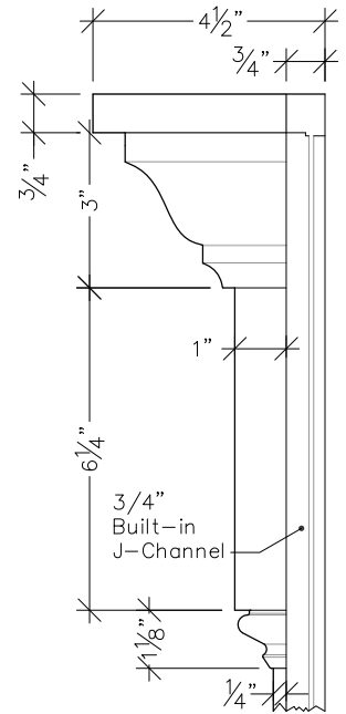
Detail #1 3"=1'-0"
